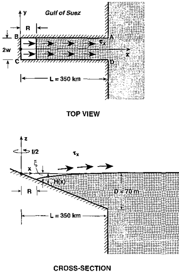
FIG. 2. Schematic diagram of the conceptual wind-crossing model. The gulf is taken to be a long and narrow channel with a linearly sloping bottom. Short, thick arrows represent the wind stress at the surface, \tau_x . The variable H(x) is the undisturbed water depth, D the maximum depth, 2w the width, L the length, and R the receding distance. Reproduced from Nof and Paldor (1992).
