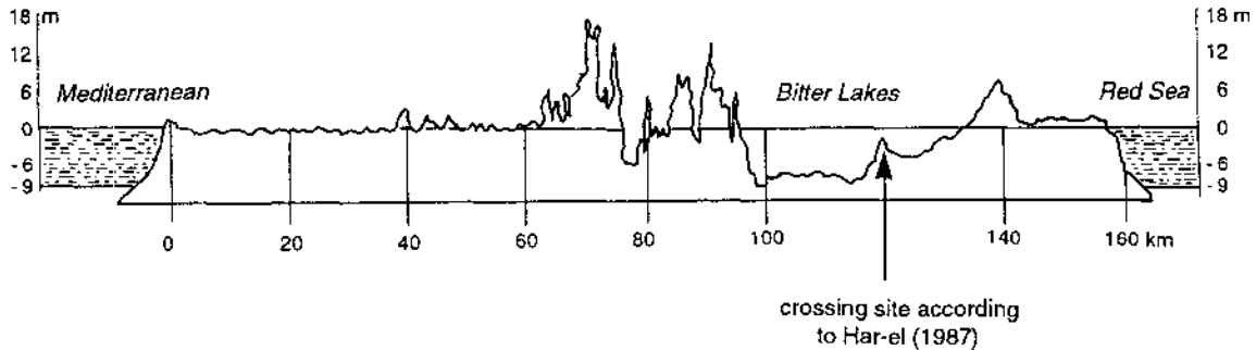
FIG. 6. A cross section from the Gulf of Suez (right) to the Mediterranean Sea (left) prior to the construction of the Suez Canal (adapted from Trumbull 1884).
